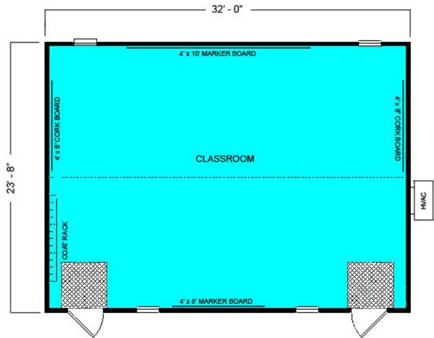
NOMINAL 24' X 32' SINGLE CLASSROOM BUILDING
