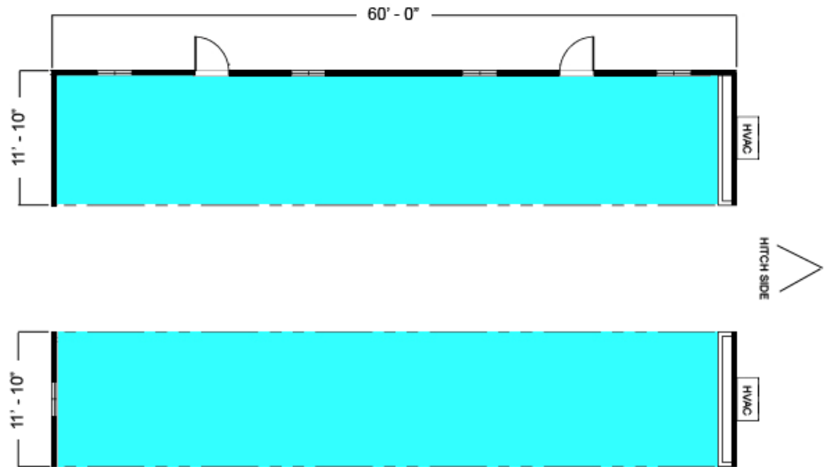
NOMINAL 12' x 60' DOH OPENS Comark Building Systems, Inc. Copyright 2007
