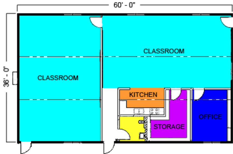
NOMINAL 36' x 60' MODULAR MULTIPURPOSE BUILDING
